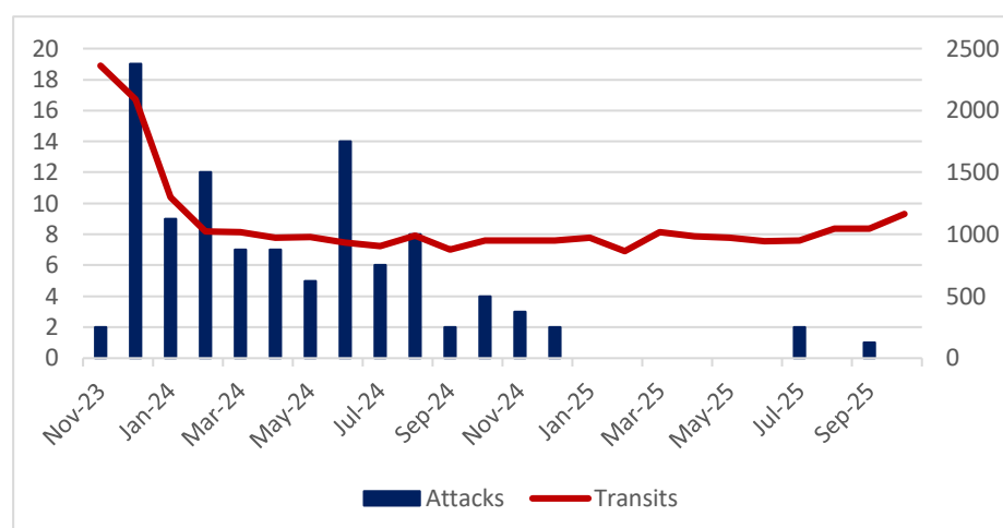
Figure 1: Attacks against merchant ships per month and number of monthly Bab el Mandeb transits by merchant ships >10,000 dwt (Source: Risk Intelligence System / Lloyd's List Intelligence/Seasearcher)
